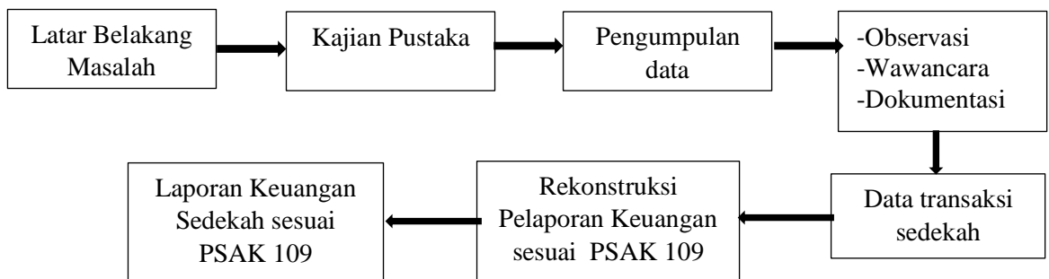
Gambar 3.2. Alur penelitian
